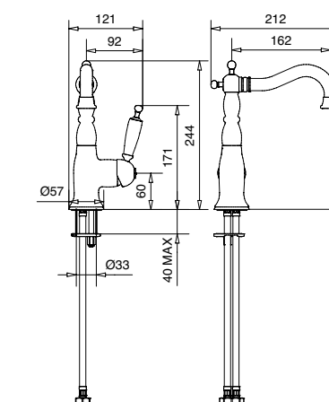
Con scarico Clic-Clac · With Clic-Clac press top waste
