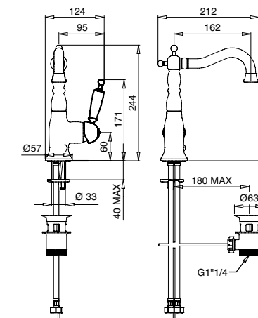
Monocomando lavabo scarico automatico 1"1/4 con flex inox Single hole basin mixer pop-up 1"1/4 with flex
